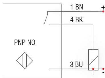
Connection diagram
