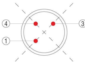
M8 connection
